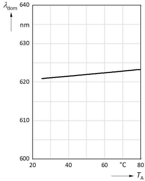
Dominant Wavelength vs. Ambiente Temperature
