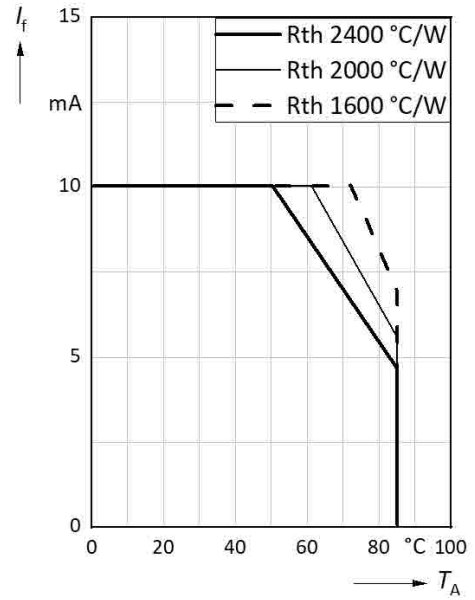
Forward Current vs. Ambiente Temperature
